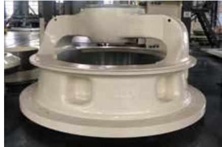
Spider Assembly
